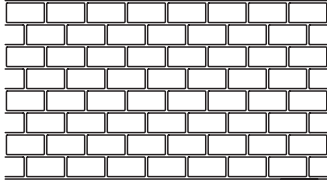
RUNNING BOND BRICK SIZE: 4'' \times 7 \frac{3}{4}'' ROLL WIDTH: 36 \frac{1}{2}'' JOINT WIDTH: \frac{1}{2}''
